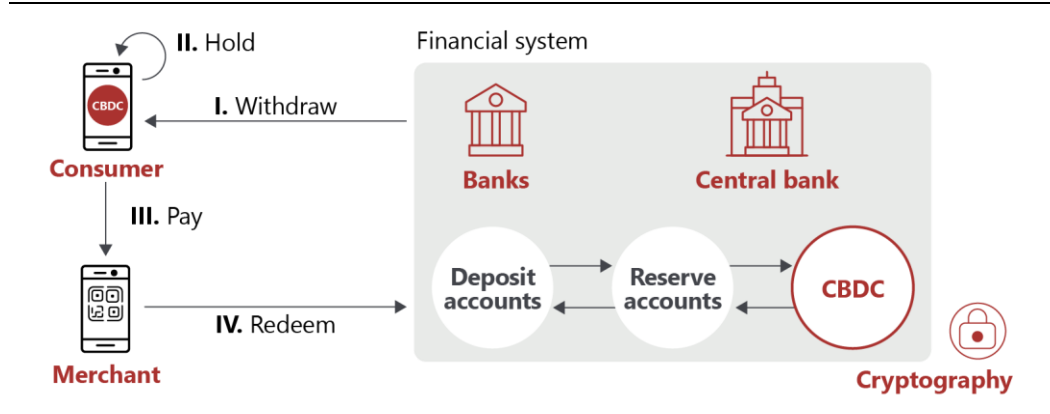
Tourbillon high-level architecture
