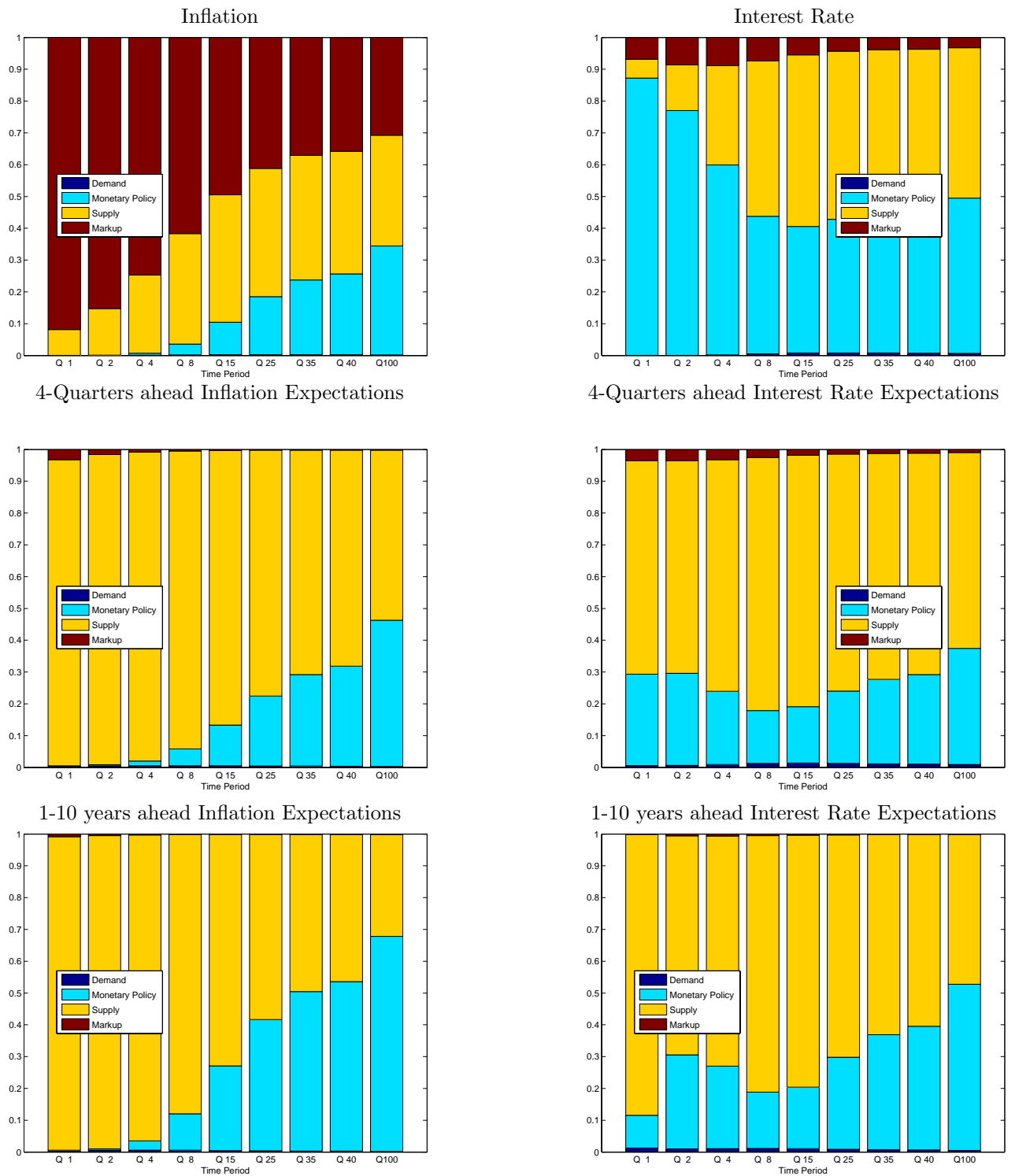
Figure 6: Variance Decomposition
