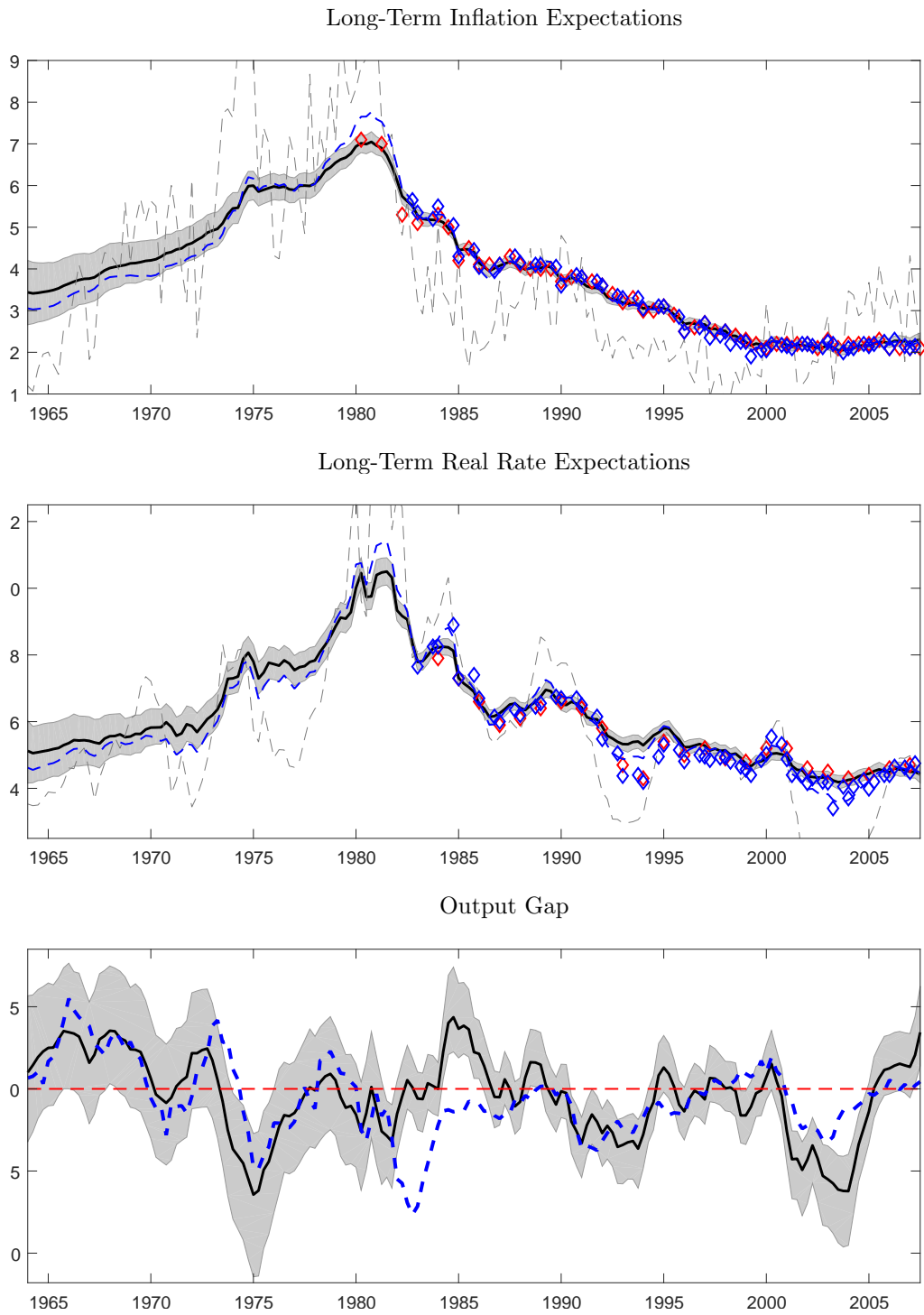
Figure 4: Baseline Predictions.
